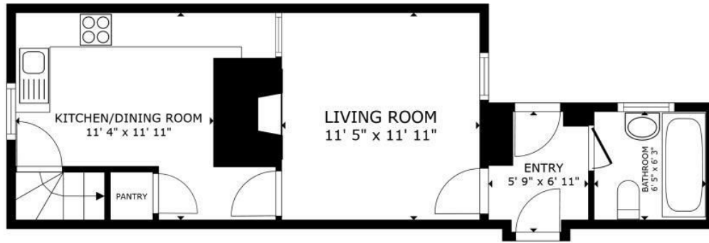
FLOOR 1
